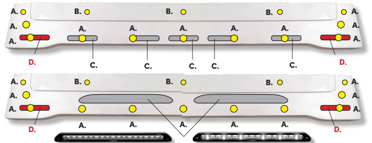
Powerful 126 W LED-bar - Lazer Linear Elite 18 with or without built in position lights
